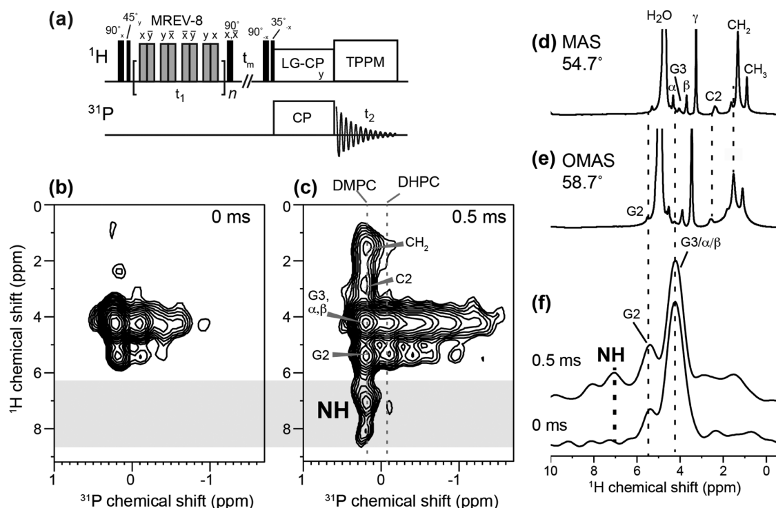
Figure 9. 2D ^{31}\text{P} - ^1\text{H} correlation spectra with ^1\text{H} homonuclear decoupling, measured at 306 K under OMAS at 58.7°. (a) Pulse sequence for the homonuclear-decoupled HETCOR experiment. (b) 2D spectrum without ^1\text{H} spin diffusion. (c) 2D spectrum with 0.5 ms ^1\text{H} spin diffusion. (d) One-dimensional ^1\text{H} MAS spectrum. (e) One-dimensional ^1\text{H} OMAS spectrum at 58.7°. (f) ^1\text{H} cross sections of DMPC with 0.5 ms (top) and 0 ms (bottom) spin diffusion, extracted from the 2D spectra in panels b and c.
