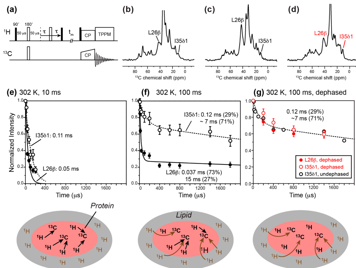
Figure 7. ^{13}\text{C} -detected ^1\text{H} T_2 relaxation data of M2TM-AH in oriented bicelles at 302 K under the static condition. (a) Pulse sequence of the dipolar-dephased ^1\text{H} T_2 relaxation experiment used to obtain the data in panel g. (b) Representative ^{13}\text{C} spectra without dipolar dephasing, measured with 10 ms ^1\text{H} spin diffusion. (c) Representative ^{13}\text{C} spectra without dipolar dephasing, measured with 100 ms ^1\text{H} spin diffusion. (d) Representative ^{13}\text{C} spectra with dipolar dephasing and 100 ms ^1\text{H} spin diffusion. The echo delay is 0 for all the spectra in panels b–d. (e) ^{13}\text{C} -detected ^1\text{H} T_2 relaxation curves with 10 ms spin diffusion. The schematic illustration below indicates that ^1\text{H} magnetization transfer is mostly within the peptide at this mixing time. (f) ^{13}\text{C} -detected ^1\text{H} T_2 relaxation curves after 100 ms spin diffusion. At this mixing time, lipid ^1\text{H} magnetization from the surrounding environment is transferred to the peptide, thus giving much slower relaxation. A fast initial decay is especially pronounced for the L26 \text{C}\beta signal. (g) ^1\text{H} T_2 relaxation curves measured with 100 \mu\text{s} C–H dipolar dephasing and 100 ms spin diffusion, to selectively detect the T_2 relaxation of lipids near the peptide. The disappearance of the fast initial decay of the L26 \text{C}\beta data verifies that the origin of the fast initial decay is the rigid peptide protons.
