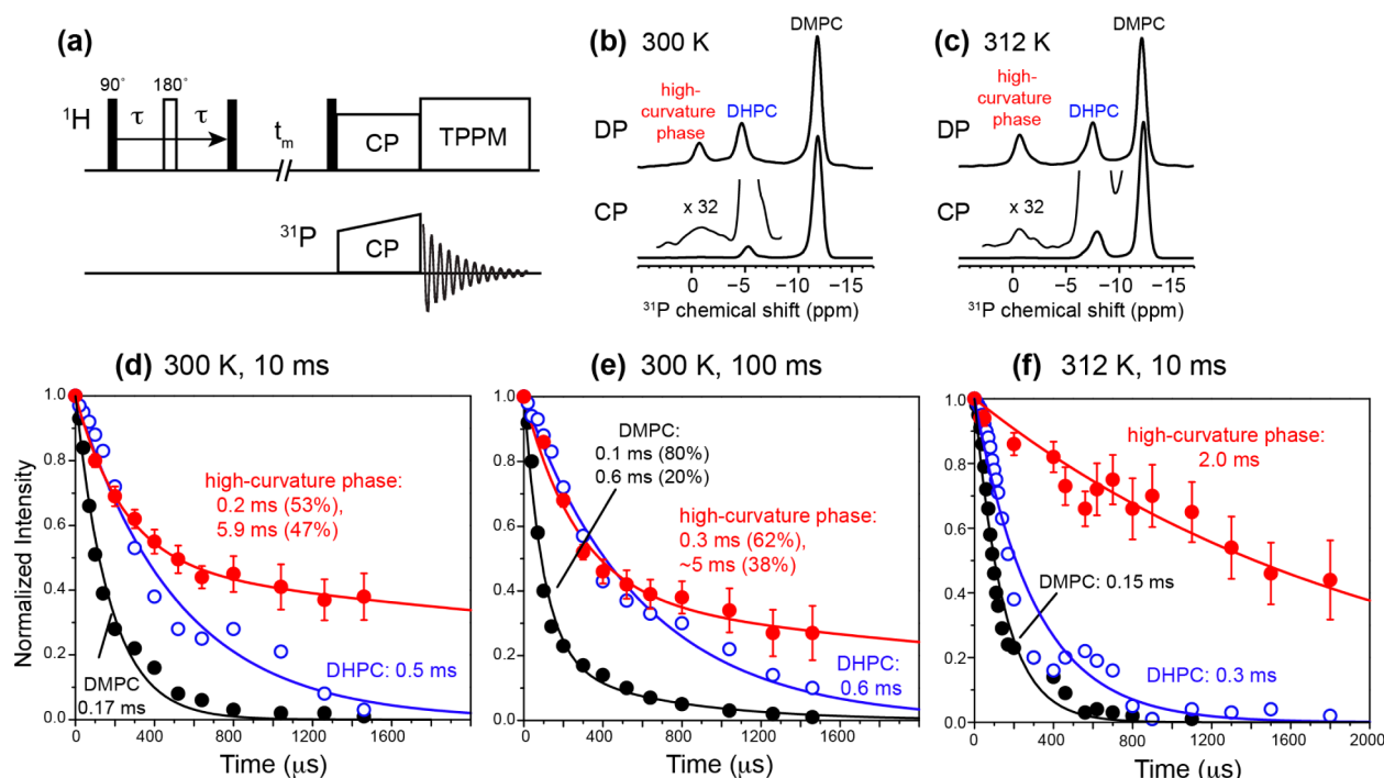
Figure 5. ^{31}\text{P} -detected ^1\text{H} T_2 relaxation data of DMPC/DHPC bicelles containing M2TM-AH under the static condition. (a) Pulse sequence of the indirectly detected ^1\text{H} T_2 experiment. (b) Representative ^{31}\text{P} DP and CP spectra with ^1\text{H} spin diffusion mixing at 300 K. (c) Representative ^{31}\text{P} DP and CP spectra with ^1\text{H} spin diffusion at 312 K. The ^{31}\text{P} chemical shifts differ between 300 and 312 K for DMPC and DHPC peaks because of temperature-dependent exchange of DHPC between the planar and edge regions of the bicelle. (d) ^1\text{H} T_2 relaxation decays at 300 K after 10 ms ^1\text{H} spin diffusion. (e) ^1\text{H} T_2 relaxation decays at 300 K after 100 ms ^1\text{H} spin diffusion. (f) ^1\text{H} T_2 relaxation decays at 312 K after 10 ms spin diffusion. The DMPC, DHPC, and high-curvature phase data are colored black, blue, and red, respectively.
