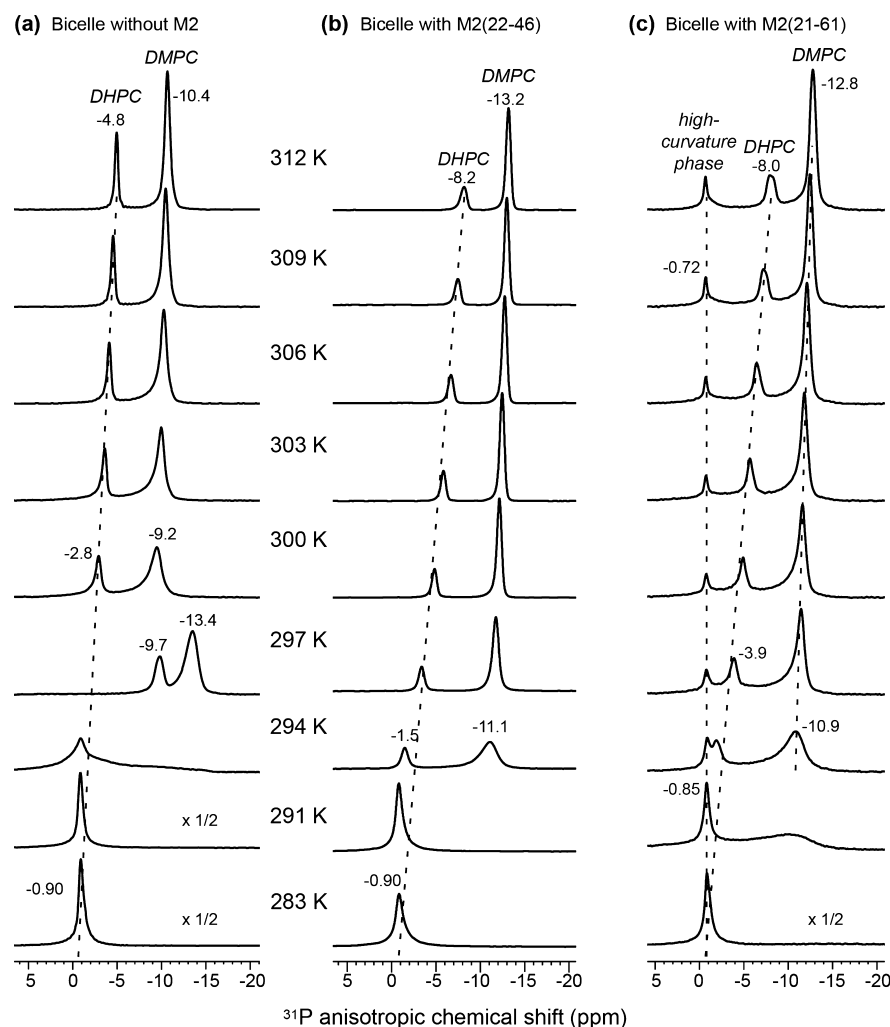
Figure 1. Variable-temperature ^{31}\text{P} spectra of static DMPC/DHPC (3:1) bicelles with and without M2. (a) Bicelles without protein. (b) Bicelle with M2TM. (c) Bicelle with M2TM-AH. M2TM-AH creates a temperature-independent isotropic ^{31}\text{P} peak, indicating the formation of a high-curvature membrane phase. The other ^{31}\text{P} chemical shifts are anisotropic and change with temperature.
