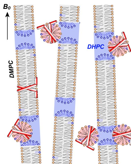
Figure 10. Schematic of M2TM-AH binding to membranes with mixed curvatures. The peptide creates a high-curvature phase that is partially associated with the round caps of bicelles. Depicted here are micelles, but bicontinuous cubic phases cannot be ruled out. Most of the peptide binds to this high-curvature phase, while a small fraction resides in the planar region of the bicelle because of its stabilization of the hydrophobic TM helix. For simplicity, only two of the four molecules of the tetrameric protein are represented.
