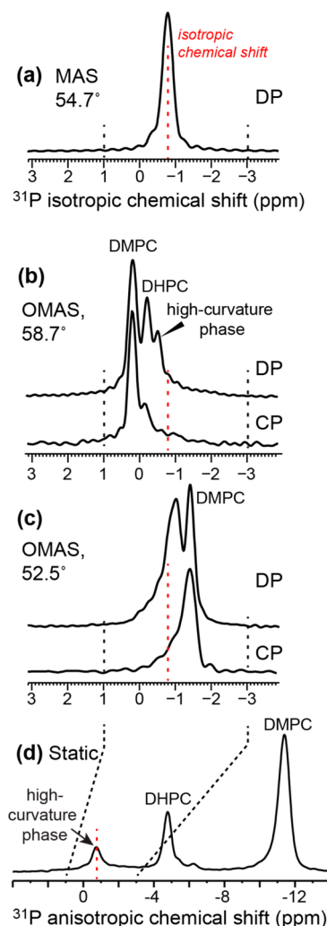
Figure 8. One-dimensional ^{31}\text{P} spectra of bicelles containing M2TM-AH under 3.5 kHz spinning at 300 K. (a) ^{31}\text{P} DP MAS spectrum. (b) ^{31}\text{P} DP and CP spectra under OMAS at 58.7^\circ . Three ^{31}\text{P} peaks are resolved. (c) ^{31}\text{P} DP and CP spectra under OMAS at 52.5^\circ . (d) Comparative static ^{31}\text{P} spectrum, showing three well-resolved peaks.
