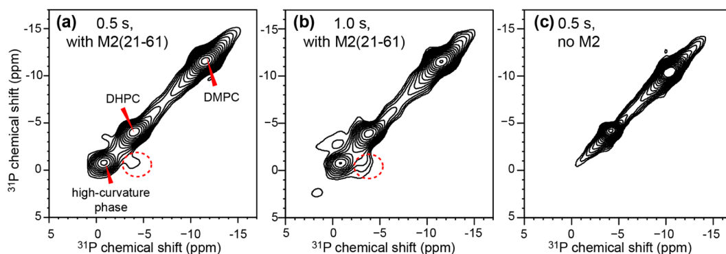
Figure 3. 2D ^{31}\text{P} – ^{31}\text{P} exchange spectra of static DMPC/DHPC bicelles. (a) With M2TM-AH and 0.5 s spin diffusion. (b) With M2TM-AH and 1.0 s spin diffusion. (c) Without M2 and with 0.5 s spin diffusion. The spectra were measured at 297 K (a and b) and 306 K (c) to obtain the same DHPC ^{31}\text{P} chemical shift. Cross-peaks between the isotropic peak and the DHPC peak (dotted circle) are observed for the protein-bound bicelles in panels a and b.
