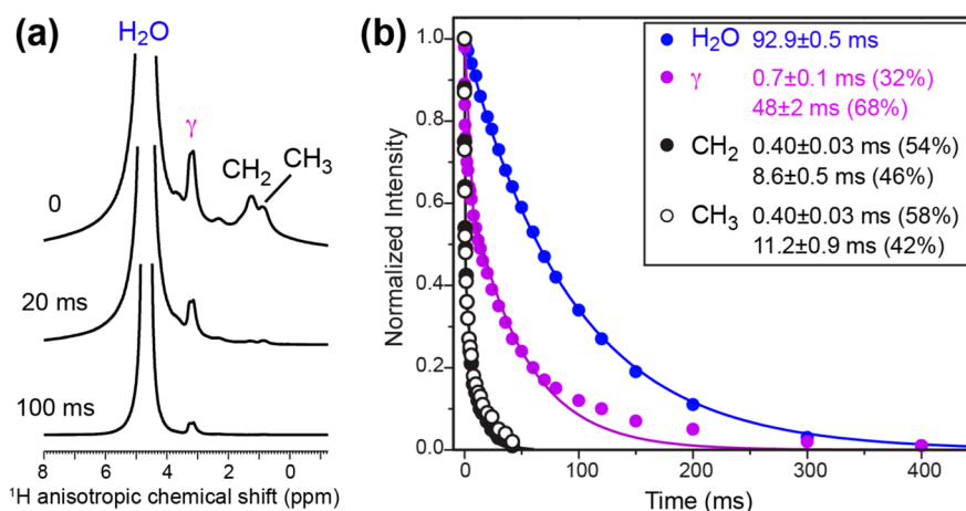
Figure 6. Directly detected ^1\text{H} T_2 relaxation data of DMPC/DHPC bicelles containing M2TM-AH under the static condition at 302 K. (a) Representative ^1\text{H} spectra with different echo delays. (b) ^1\text{H} T_2 relaxation curves with single- or double-exponential fits. The decay constants and the corresponding fractions are listed. The lipid relaxation times range from 0.4 to 50 ms, whereas the water ^1\text{H} T_2 relaxation time is much longer, 93 ms.
