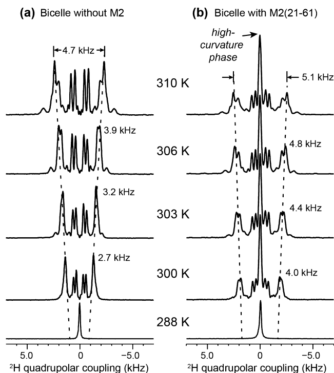
Figure 2. Static ^2\text{H} spectra of d_{22} -DHPC in DMPC/DHPC bicelles. (a) Bicelles without the peptide. (b) Bicelles with M2TM-AH. The peptide-bound membrane shows a zero-frequency peak, indicating the presence of an isotropic membrane domain or a bicontinuous cubic phase.
